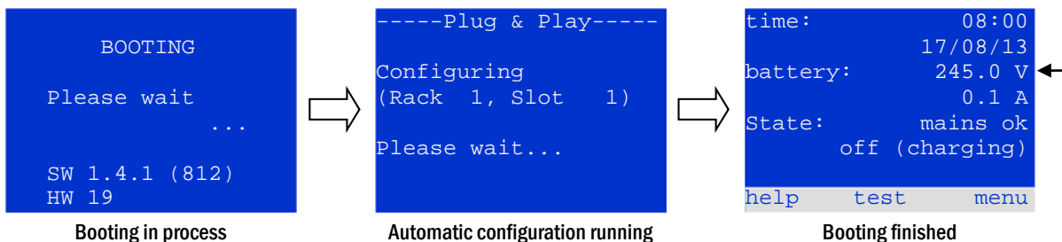
Figure 19: Boot process (left, middle) and status message (right).
