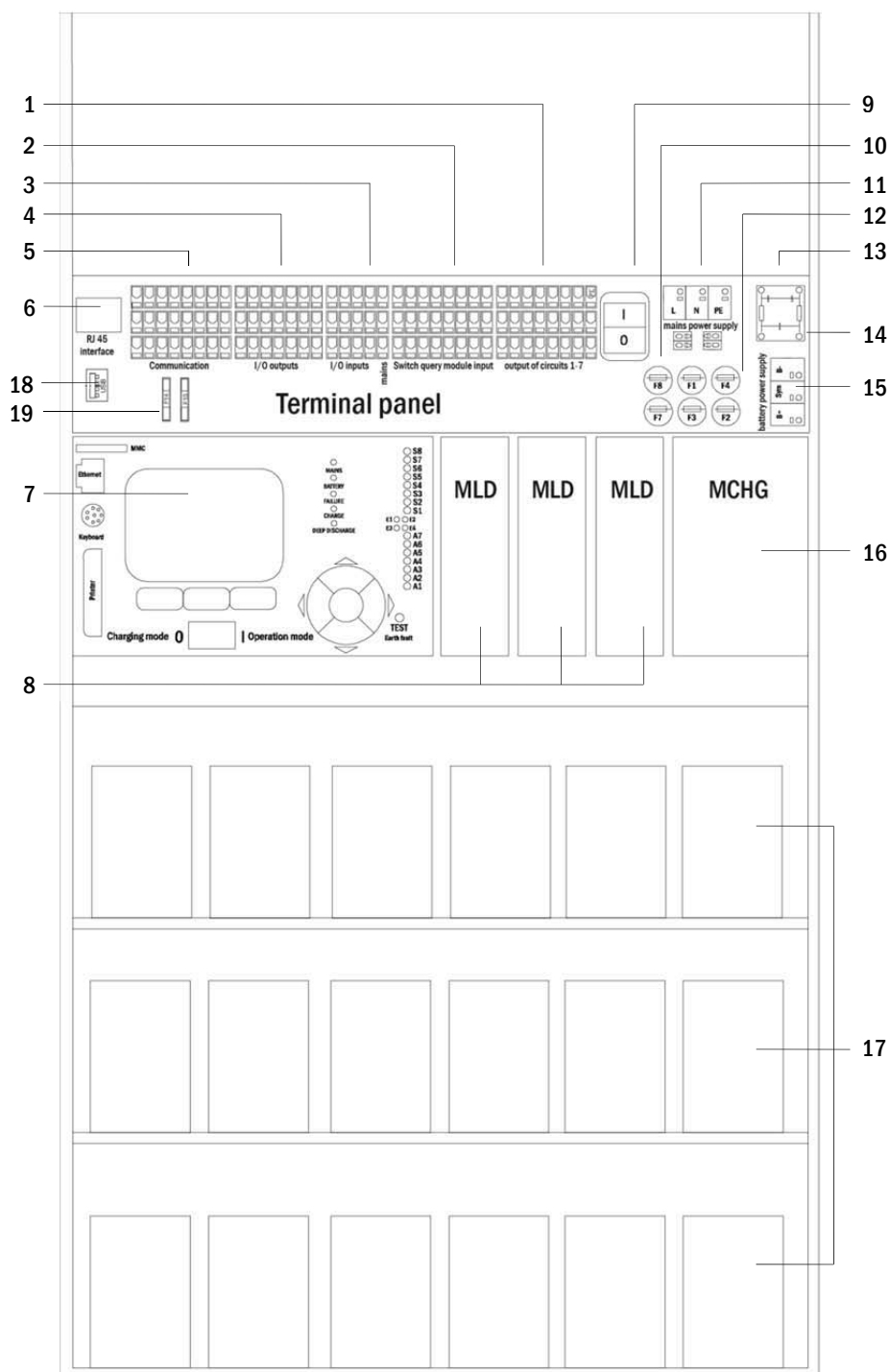
Figure 1: vista interna
