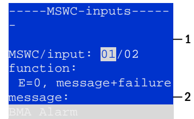
Figure 62: Programming of the MSWC-inputs
