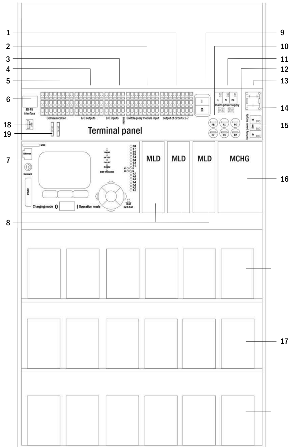
Figure 1: Inside view
