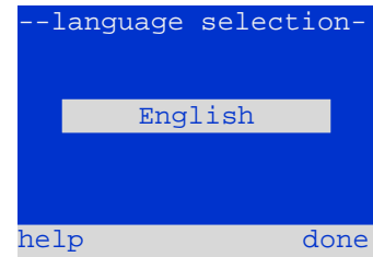
Figure 64: Language selection
