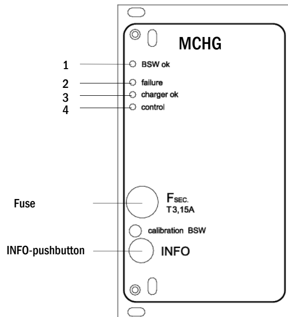
Figure 17: Charger module
