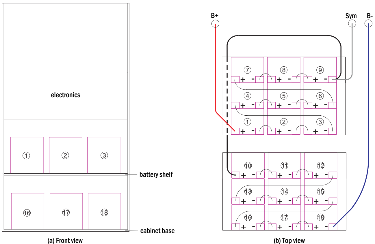
Figure 14: Mounting and connection of the battery blocks 12V 5.2Ah
