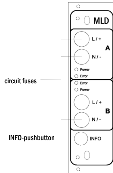
Figure 16: MLD- module
