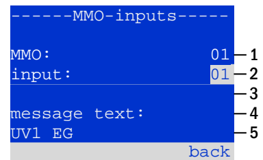
Figure 63: Programming of the MMO-inputs
