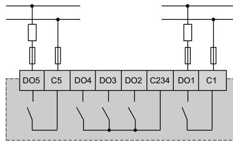
TM173ODM22S (CN6) SSR output:
