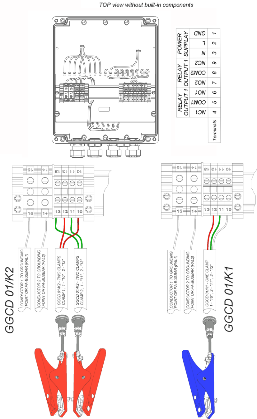
Electric connection scheme of cables and conductors:
