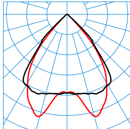
SFlow D2-L MRX LED4000-840 ETDD 03 TX723894
