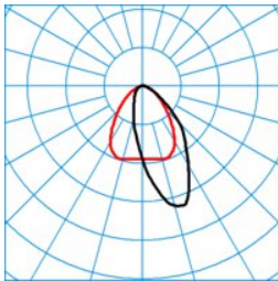
ELINE HE LAN40-120 ML 865 L150 4 20 ■ C0 - C180 DIN 5040 = A50 UTE 3 = 0.98 C + 0.02 T CEN flux code = 63 89 98 98 100 0 6 44 2
