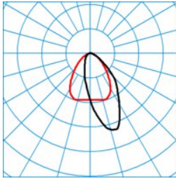
ELINE HE LAN40-120 ML 865 L150 2 20 ■ C0 - C180 DIN 5040 = A50 UTE 3 = 0.98 C + 0.02 T CEN flux code = 63 89 98 98 100 0 6 44 2
