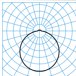
Olisq RWD4 DW 40-840 ETBLE +CAS TX565830
