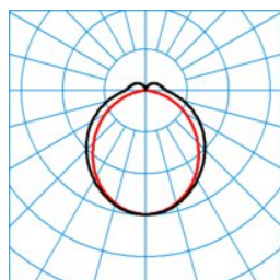
ELINE DL35-100 ML 840 L150 4 50
