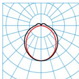
ELINE DL35-100 ML 840 L150 2 50
