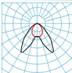
ELINE HE LDAH60-160 ML 865 L225 0 50 ■ C0 - C180
