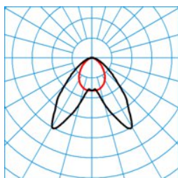
ELINE HE LDAH60-160 ML 865 L225 4 50 ■ C0 - C180
