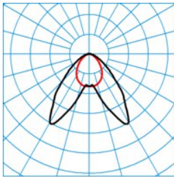
ELINE HE LDAW60-160 ML 865 L225 2 50 ■ C0 - C180
