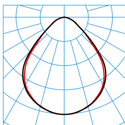
Opendo D1-L PW19 20-36/4/ML-840 ET 03 (3600lm) TX376524
