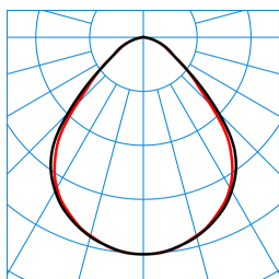
Opendo D1-L PW19 20-36/4/ML-840 ET 03 (2500lm) TX376522
