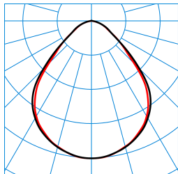
Opendo D1-L PW19 20-36/4/ML-840 ET 03 (2000lm) TX376521
