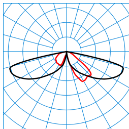
CS 19 100-AB2L/2900-740 2G1S ETDD (CLO initial value) TX299975
