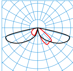
CS 19 100-AB2L/2900-740 2G1S ETDD (CLO end value) TX299974
