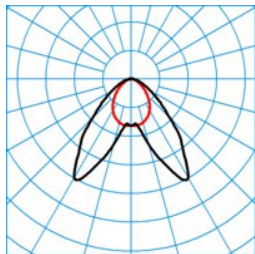
ELINE LDAW40-110 ML 840 L150 0 20 ■ C0 - C180
