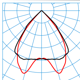
SFLOW C3-L MRX 40-830 ETBLE +CAS-S 01 TX562373
