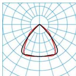
ELINE LW2240-110 ML 865 L150 2 20 ■ C0 - C180
