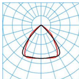
ELINE LW2240-110 ML 865 L150 0 20 ■ C0 - C180
