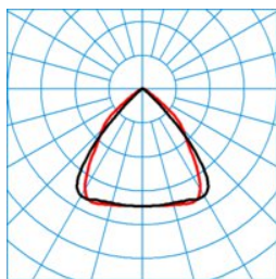
ELINE HE LW2240-120 ML 865 L150 4 20 ■ C0 - C180
