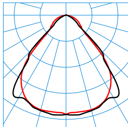
SFlow C2-L MRW LED4000-840 ET 01 TX721239
