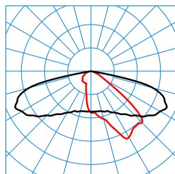
LIQ 50N-AB2L-LR/4200-727 6G1 ET (CLO initial value) TX777857
