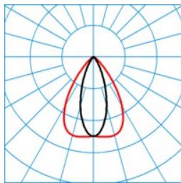
ELINE HE LVN60-160 ML 830 L225 2 20 ■ C0 - C180
