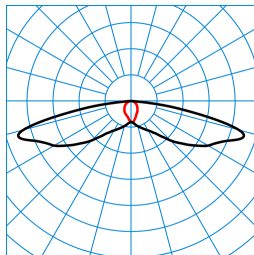
LIQ 50N-SB3L-LRA/1650-722 2G1 ETDD (CLO initial value) TX780091
