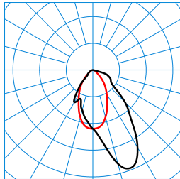
Creavo M46-TS LWW-03 42-840 ETDD 01 TX775386
