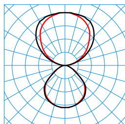
Luceos D/H1-L CDP 4000-8TW ETDD 03 (Pendant ZS/ZST) (CCW) TX877231
