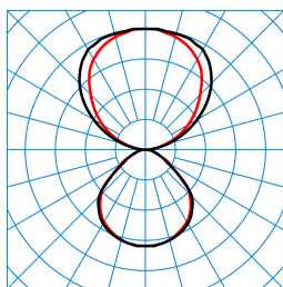
Luceos D/H1-L CDP 4000-8TW ETDD 03 (Pendant ZS/ZST) (CSU) TX877232
