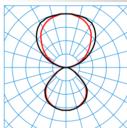
Luceos D/H1-L CDP 4000-8TW ETDD 03 (Pendant ZS/ZST) (CWW) TX877233
