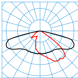
LIQ 70N-AB7L-LR/16000-730 12G1 ET (CLO initial value) TX778262
