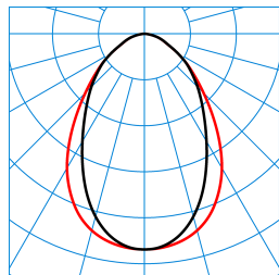
ArimoFit M46 DW19 42-8TW ETDD8 (DSU) TX874779
