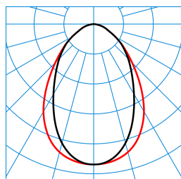
ArimoFit M46 DW19 42-8TW ETDD8 + ArimoFit Sky M46-TS ZER (DSU) TX874773
