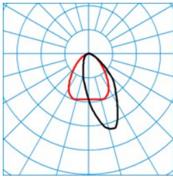
ELINE HE LAN40-120 ML 830 L150 2 20 ■ C0 - C180 DIN 5040 = A50 UTE 3 = 0.98 C + 0.02 T CEN flux code = 63 89 98 98 100 0 6 44 2
