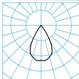
SNS QC3-WR1VFL-14-840
