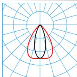
ELINE LVN40-110 ML 830 L150 0 50
