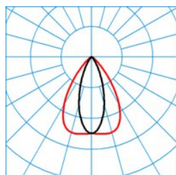
ELINE LVN40-110 ML 830 L150 4 50
