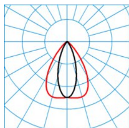
ELINE LVN40-110 ML 830 L150 2 50
