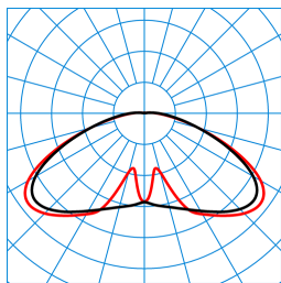
Publisca P1W-RBT/1500-740 2G1S ETDD (CLO end value) TX301017
