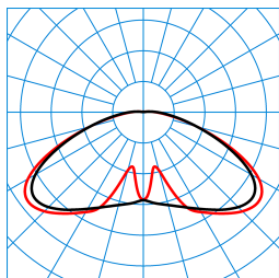
Publisca P1W-RBT/1500-740 2G1S ETDD (CLO initial value) TX301946
