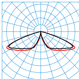
CS 19 C 100-RB6L/1800-740 2G1S ETDD (CLO initial value) TX300167
