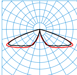
CS 19 C 100-RB6L/1800-740 2G1S ETDD (CLO end value) TX300166
