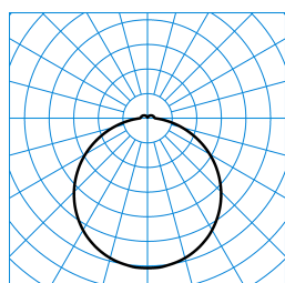
Olisq RWD2 DW 20-8TW ETBLE +CAS-S + RWD2 ZDR 1/2 03 (DWW) TX873510
