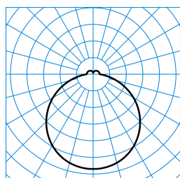
Olisq RWD2 DW 20-8TW ETBLE +CAS-S (DCW) TX873490
