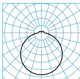
Olisq RWD2 DW 20-8TW ETBLE +CAS-S (DSU) TX873491
