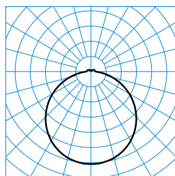
Olisq RWD2 DW 20-8TW ETBLE +CAS-S + RWD2 ZDR 1/2 05 (DWW) TX873513
