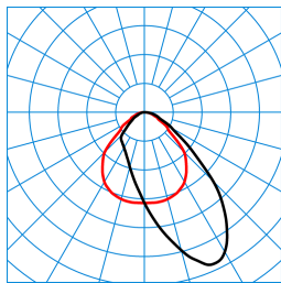
Luceos D/H2-L CDP-A 5000-840 ETDD 01 (Pendant ZS/ZST) TX877271
