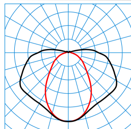
Acquex LED-M 0.6 20-840 ETDD PC TX774483
