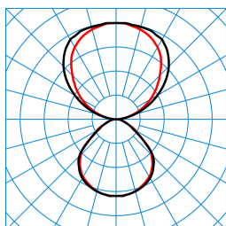
Luceos D/H2-L CDP 6500-840 ETDD 01 (Pendant ZS/ZST+EB3) TX245960
