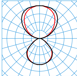
Luceos D/H2-L CDP 6500-840 ETDD 01 (Pendant ZS/ZST) TX877259
