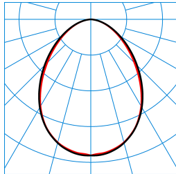
SFlow D2-L MRWD LED4000-840 ETDD 01 TX770128
