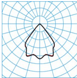
ELINE HE CLW2240-120 ML 840 L225 4 20 ■ C0 - C180 DIN 5040 = A60 UGR I 3 = 21,0 UGR q 3 = 21,0 UTE 3 = 1.00 A CEN flux code = 89 100 100 100 100
