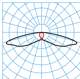
LIQ 50N-SB3L-LR/1200-722 2G1 ET (CLO initial value) TX779554
