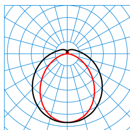
So-Tube G3 D/H3 DW 30-8TW ETDD 05 (DSU) TX874891
