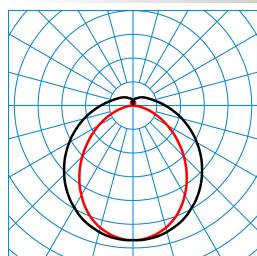
So-Tube G3 D/H3 DW 30-8TW ETDD 05 (DCW) TX874890
