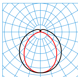
So-Tube G3 D/H3 DW 30-8TW ETDD 05 (DWW) TX874892
