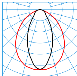
Nextrema G3 HE TB 130-840 ETDD +LV TWP TX768648
