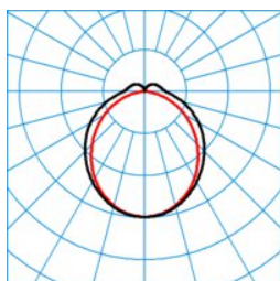
ELINE DL35-100 ML 865 L150 2 50
