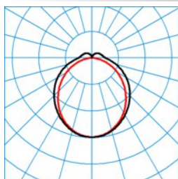
ELINE DL35-100 ML 865 L150 0 50
