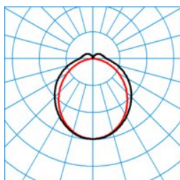
ELINE DL35-100 ML 865 L150 4 50
