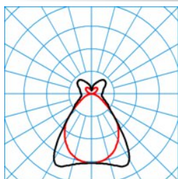
ELINE HE PMW2230-100 ML 865 L150 0 50 ■ C0 - C180
