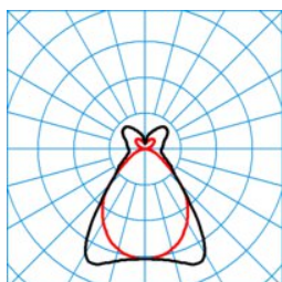
ELINE HE PMW2230-100 ML 865 L150 2 50 ■ C0 - C180
