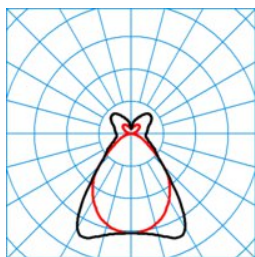
ELINE HE PMW2230-100 ML 865 L150 4 50 C0 - C180
