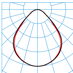
Opendo D2-L PW19 47-8TW ETBLE +CAS 01 (DSU) TX874518
