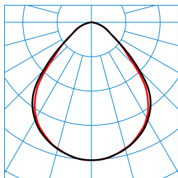
Opendo D2-L PW19 47-8TW ETBLE +CAS 01 (DWW) TX874519
