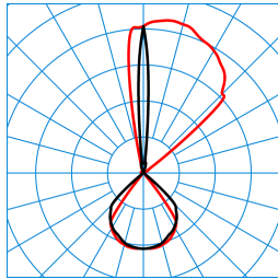
Skeo Q-W1-DI GT AM4R-RB9R/100-830 ET TX773780
