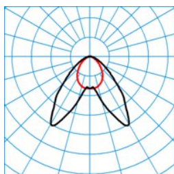
ELINE HE LDAH60-160 ML 830 L225 2 50 ■ C0 - C180
