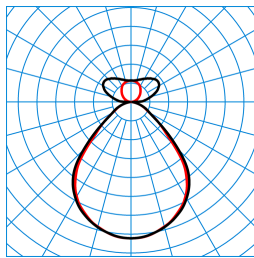
Opendo H2-L PW19 64-840 ETDD +LLWM 03 TX277425
