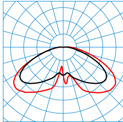
Publisca P1W-RBT/2200-730 3G1S TX053559
