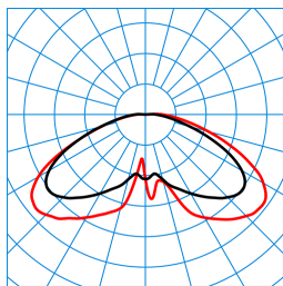
Publisca P1W-RBT/2200-730 3G1S ETDD (CLO end value) TX301567
