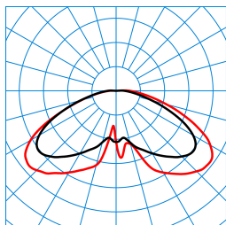
Publisca P1W-RBT/2200-730 3G1S ETDD (CLO initial value) TX300560
