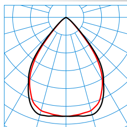
Creavo M57-TS LW19-03 42-8TW ETBLE-S 01 (DWW) TX874539
