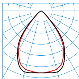
Creavo M57-TS LW19-03 42-8TW ETBLE-S 01 (DSU) TX874534
