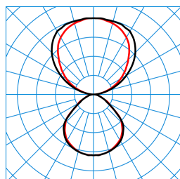
Luceos D/H2-L CDP 6500-840 ETDD 03 (Pendant ZS/ZST+EB3) TX245961
