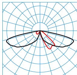
LTX P-AB2L-LRA/2600-730 3G1 ETDD TX779374
