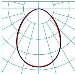
SFlow C3-L MRWD LED4000-840 ETDD LLWS 01 TX719557
