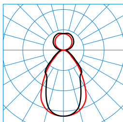
SFlow H2-L CDP-I 64-8TW ETBLE +CAS 03 (DSU) TX876373
