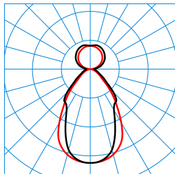
SFlow H2-L CDP-I 64-8TW ETBLE +CAS 03 (DWW) TX876413
