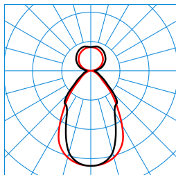
SFlow H2-L CDP-I 64-8TW ETBLE +CAS 03 (DCW) TX876398
