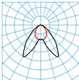
ELINE LDAH40-110 ML 830 L150 4 50
