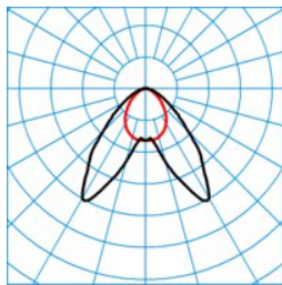
ELINE LDAH40-110 ML 830 L150 2 50
