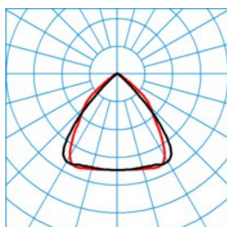
ELINE LW2240-110 ML 865 L150 4 50 ■ C0 - C180
