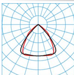
ELINE LW2240-110 ML 865 L150 0 50 ■ C0 - C180
