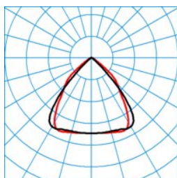
ELINE LW2240-110 ML 865 L150 2 50 ■ C0 - C180
