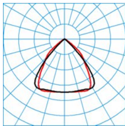
ELINE LW2240-110 ML 865 L150 2 50
